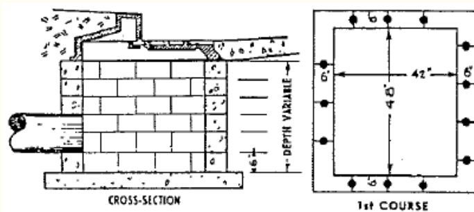
Catch Basin
