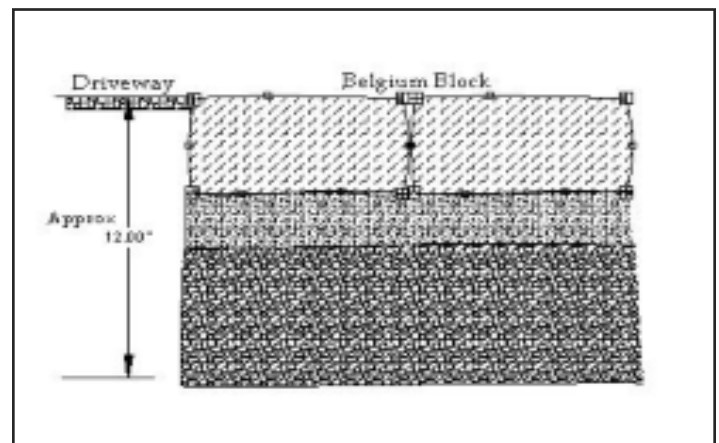
Typical Paving Detail
