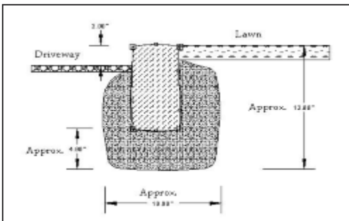
Typical Edging Detail
