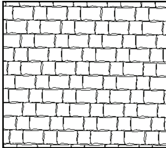
Running Bond Staggered 6" x 6" & 6" x 9" 1.6 pcs of each size per sqft
