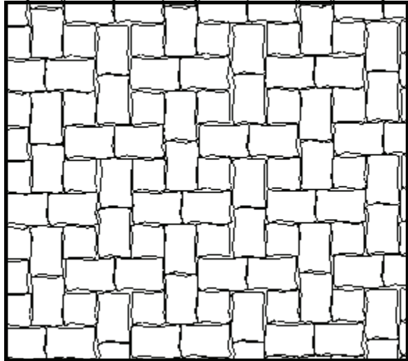
T Pattern - 2 pcs 6" x 9" & 1 pc 6" x 6" per sqft
