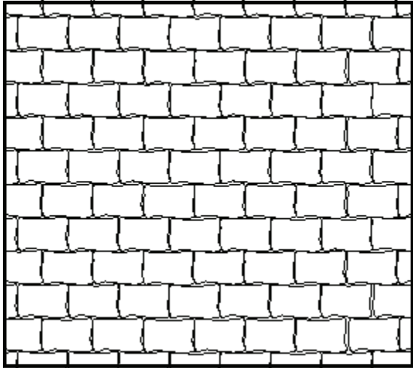
Running Bond 2.67 pcs 6" x 9" per sqft
