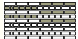
English Bond
