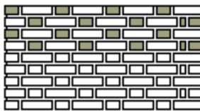
Flemish Bond
