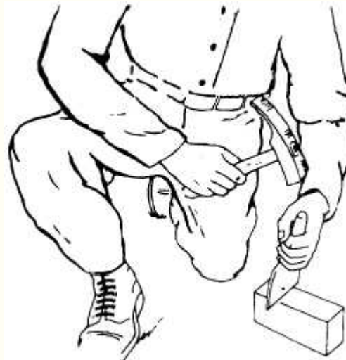
CUTTING BRICK WITH A CHISEL (FIGURE 1)
